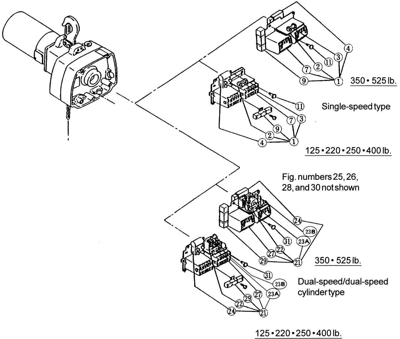
FIGURE 9-3 ELECTRIC PARTS
